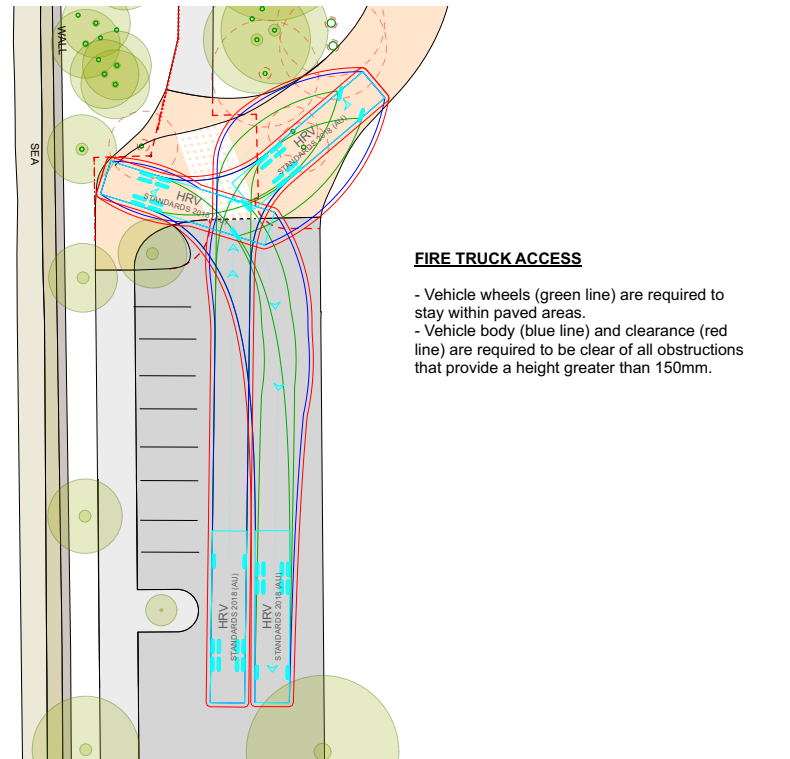
4. Swept Path-Heavy Rigid Vehicles (fire truck tested)
