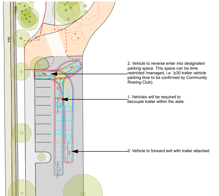
3. Swept Path-Trailer Decoupled in Aisle
